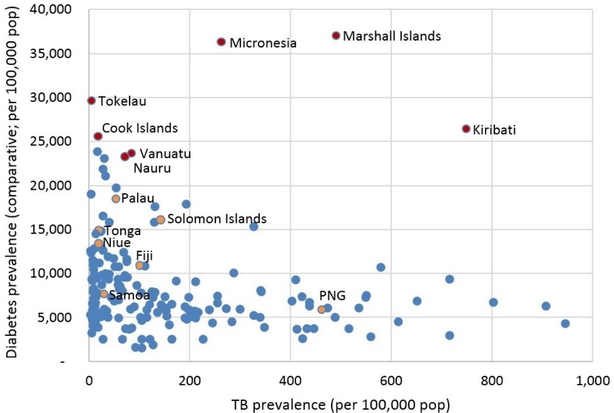
Figure 1: TB and diabetes prevalence for 195 countries
